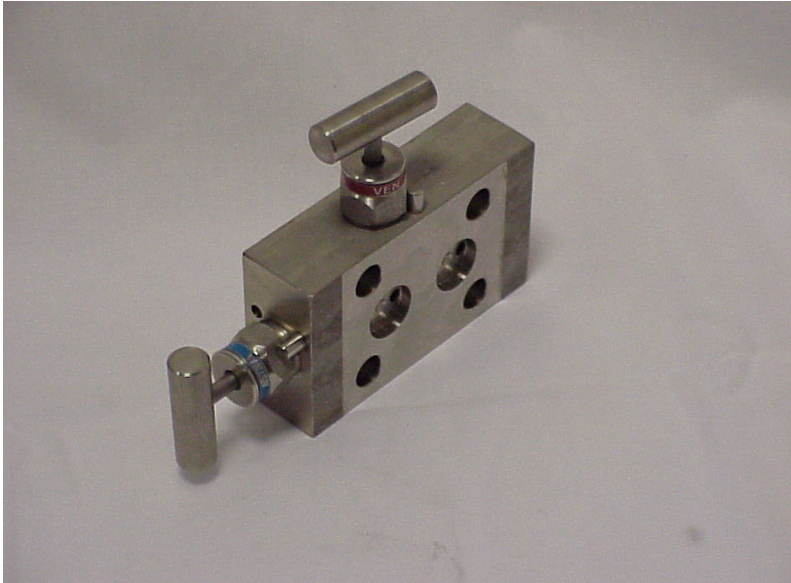
PICTURE MODEL: 246-065 2-VALVE MANIFOLD FOR DIRECT MOUNTING ON ROSEMOUNT 3051 PRESSURE TRANSMITTER WITHOUT CO-PLANAR FLANGE WITH MOUNTING BRACKET
