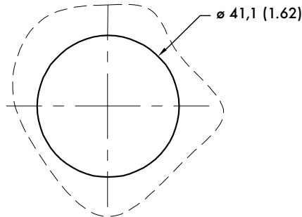
Befestigungsbohrbild/ Required mounting hole for panel mounting
