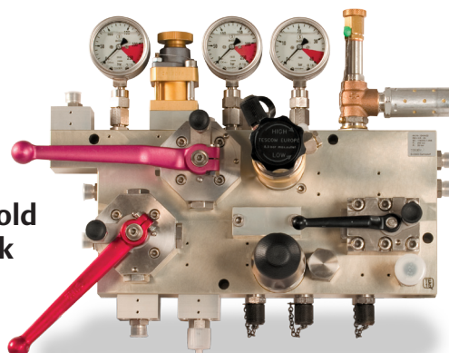
Changeover Panel
